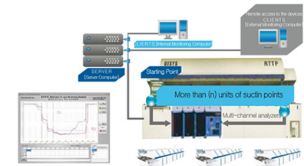
REFLOW CHECKER
