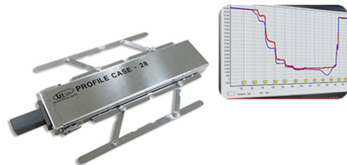
IN-LINE O2 (N2) ANALYZER
