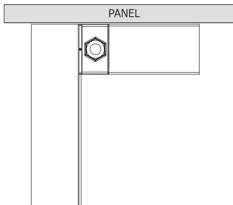
〈Panel Attachment for AL Rack assembled with Square AL Pipe〉
