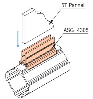
* AL Sheet Guide for Ø43
