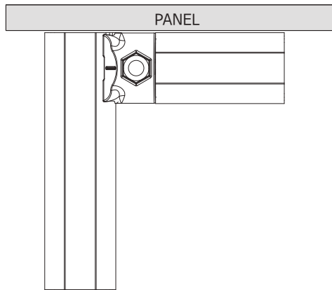
〈Panel Attachment for AL Rack assembled with Standard AL Pipe〉
